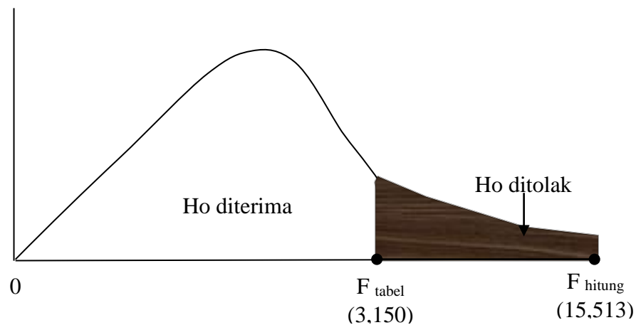
Gambar 1. Kurva Distribusi Normal F-test (Sumber: Lampiran 6, 2022)
