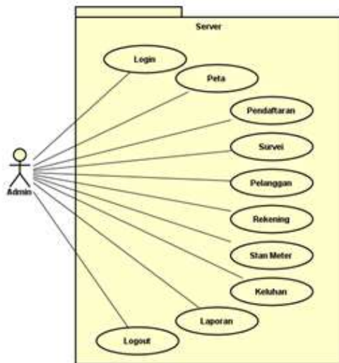
Gambar 1 Use case diagram server
