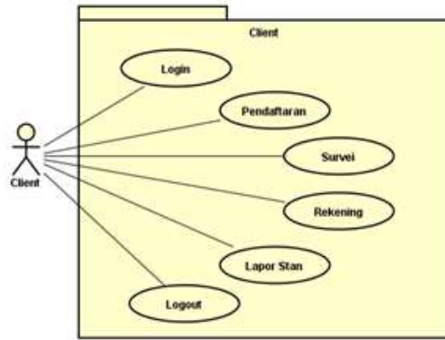
Gambar 2. Use Case diagram client
