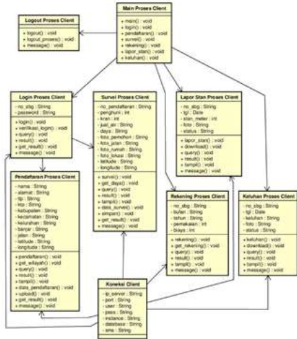
Gambar 4. Class Diagram Client
