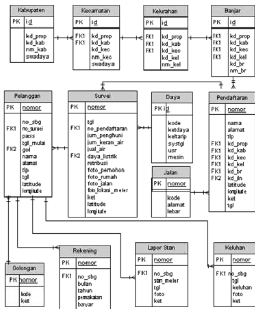
Gambar 7. Conceptual Database Server
