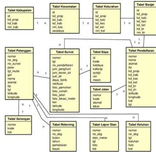
Gambar 5. Data Diagram Server
