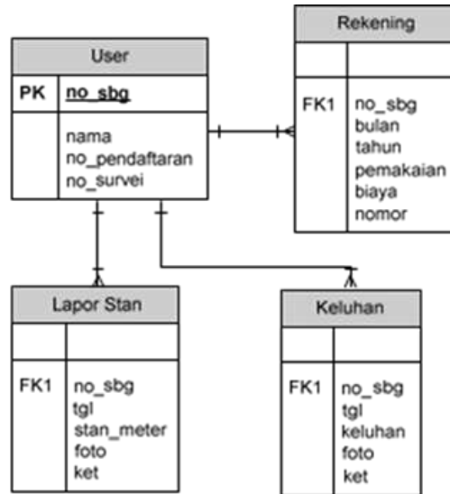
Gambar 8. Conceptual Database Client
