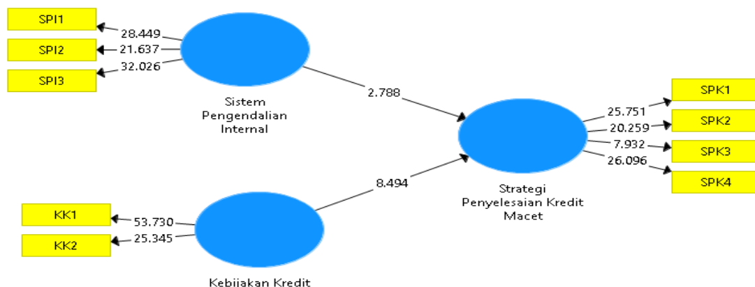
Gambar 1. Nilai Bootstraping
